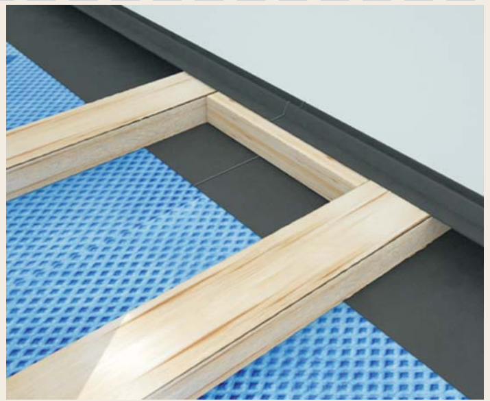
insert a batten off-cut to join easy verge together
